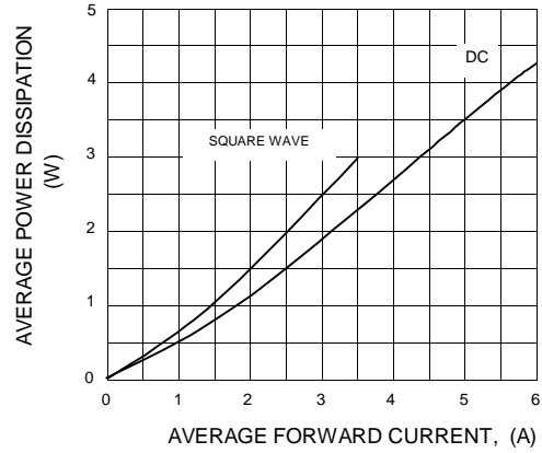
FIG.2 - POWER DISSIPATION
