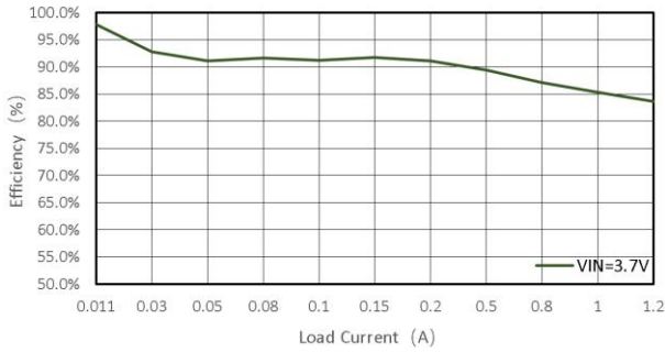
Efficiency @ Vout=5V
