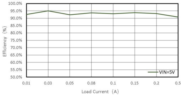
Efficiency @ Vout=12V
