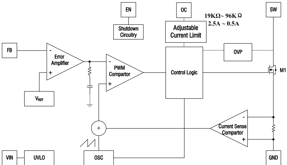
Figure 2. MFP6291LR-G1 Block Diagram
