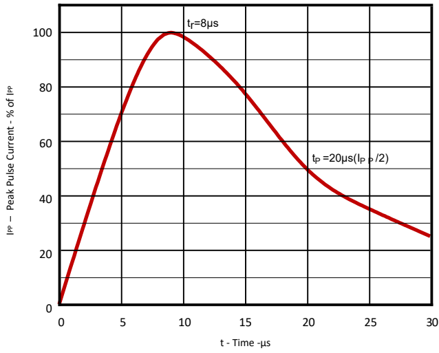
Fig 1. Pulse Waveform (8/20µs)
