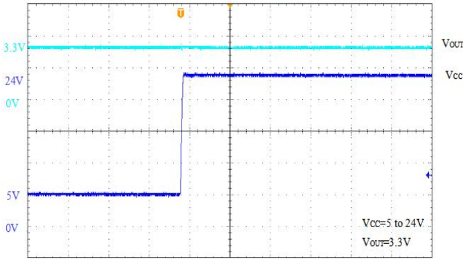
Time(4us/div)
