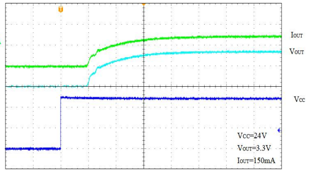
Time(100us/div)
