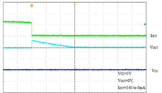
Time(200us/div)
