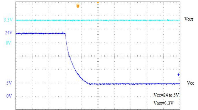
Time(4us/div)
