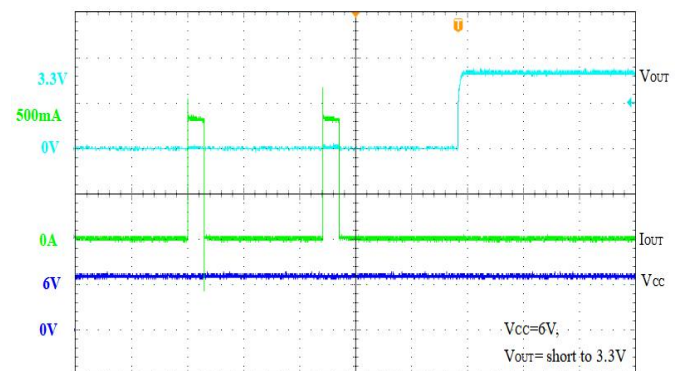
Time(2ms/div)
