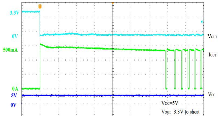
Time(20ms/div)
