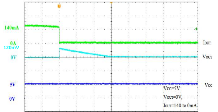
Time(200us/div)
