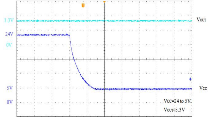
Time(4us/div)
