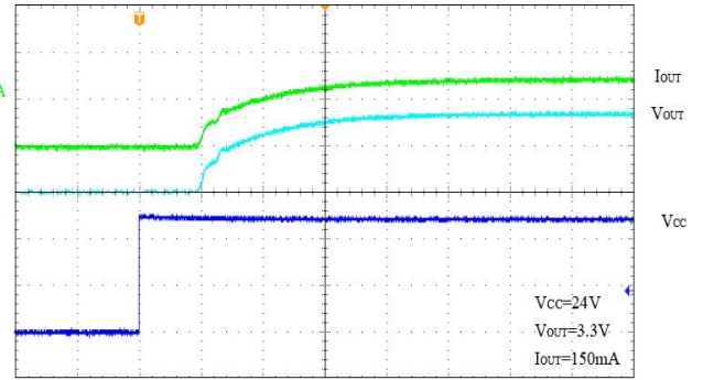
Time(100us/div)
