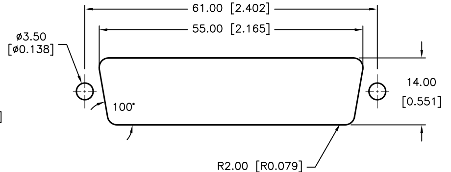
PANEL CUTOUT
