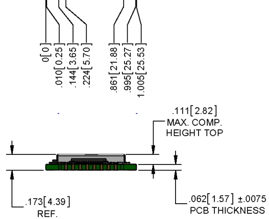
DIMENSIONS IN In [mm]
