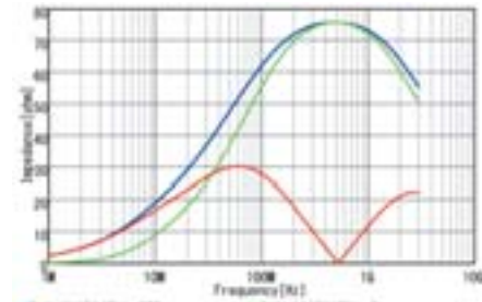
BLM18KG700TZ1/BLM18KG700TH1
