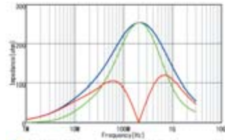
BLM18KG221SZ1/BLM18KG221SH1
