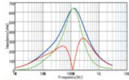
BLM18KG601SZ1/BLM18KG601SH1
