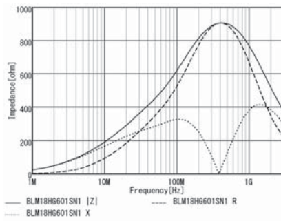
BLM18HG601SN1
