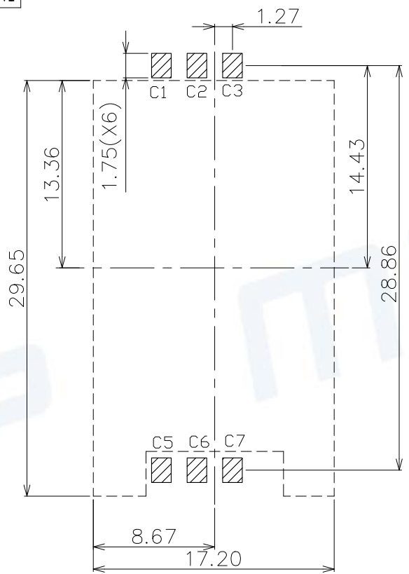
RECOMMENDED P.C.B LAYOUT COMPONENT SIDE(TOLERANCE ±0.05)
