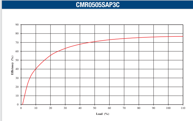
CMR0505SAP3C
