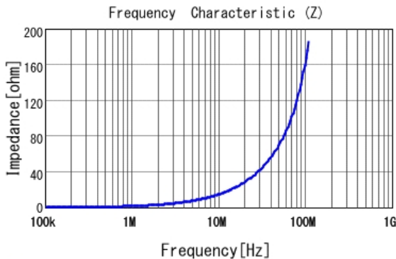
DFE201612PD-R24M |Z|
