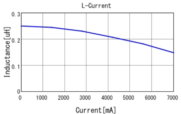
DFE201612PD-R24M L-Current 20degC
