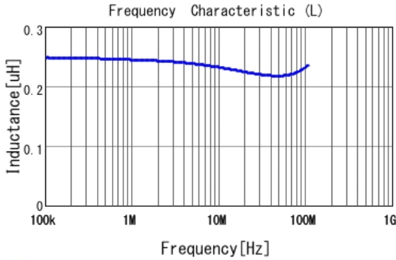
DFE201612PD-R24M L
