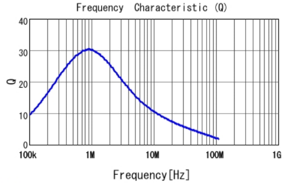
DFE201612PD-R24M Q
