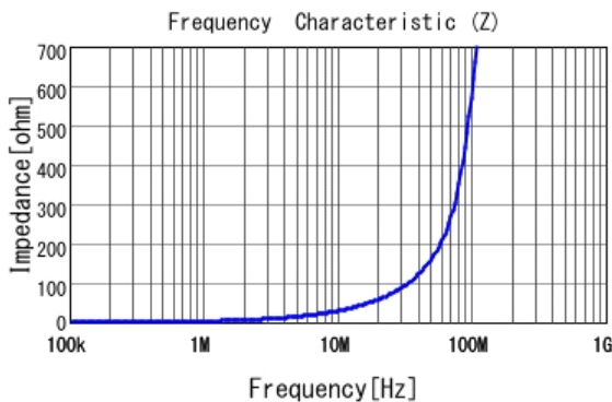
DFE201612PD-R47M |Z|
