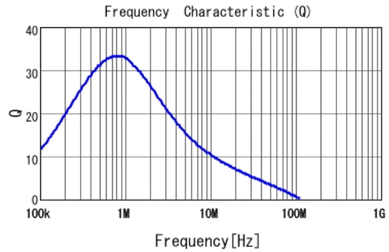
DFE201612PD-R47M Q
