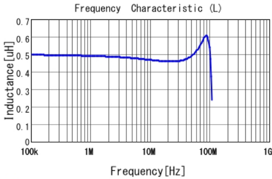
DFE201612PD-R47M L
