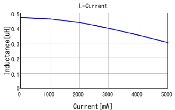
DFE201612PD-R47M L-Current 20degC
