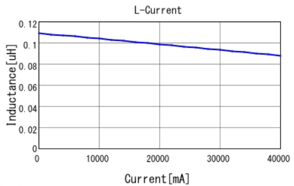
■ FDUE0630-H-R12M L-Current 20degC
