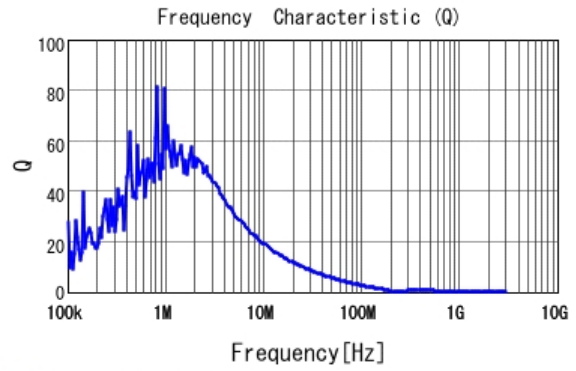
■ FDUE0630-H-R12M Q
