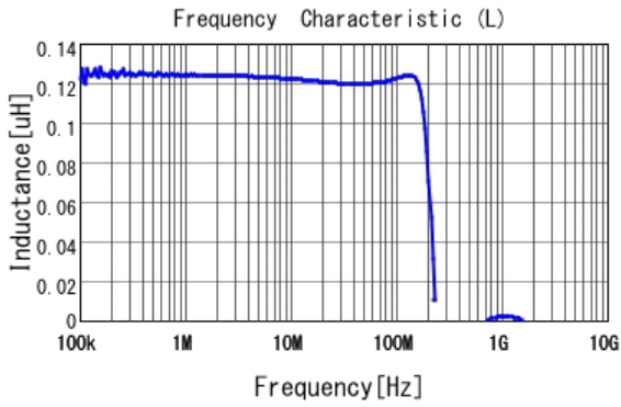
■ FDUE0630-H-R12M L
