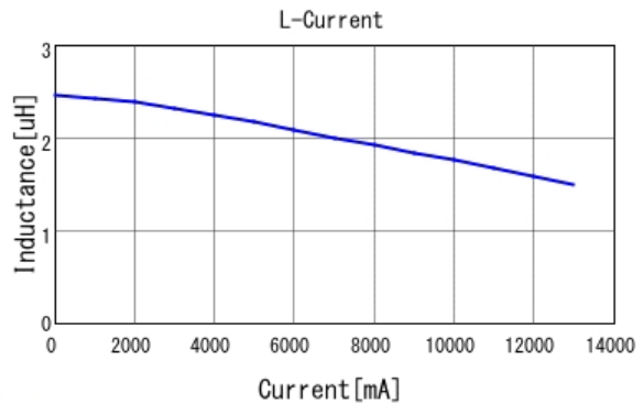
■ FDVE0640-H-2R2M L-Current 20degC
