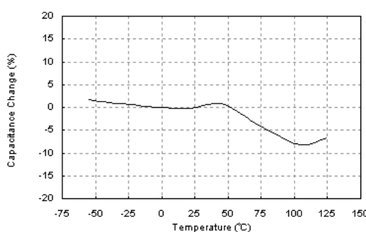
□ Typical temperature characteristics Char.R7 (X7R)
