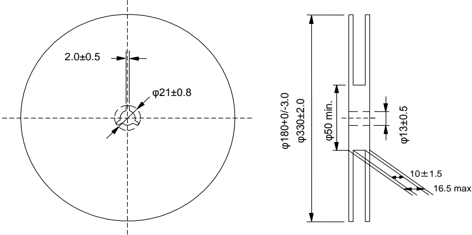
Fig.3 Taping Diagram
