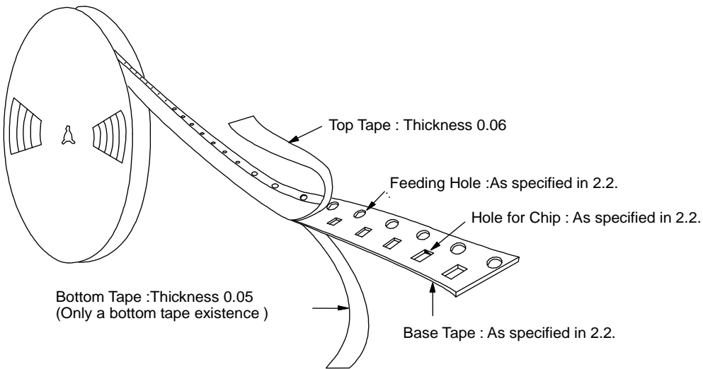
Fig.3 Taping Diagram
