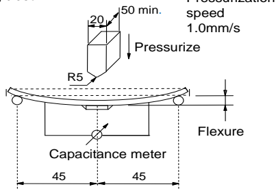
Fig.1 (in mm)
