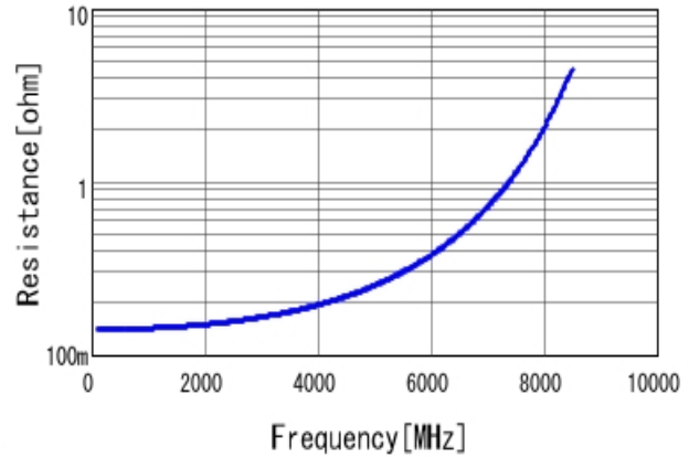
■GJM1555C1H2R6CB01 R DC0V, 25degC
