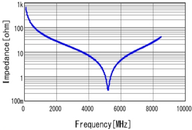
■GJM1555C1H2R6CB01 |Z| DC0V, 25degC
