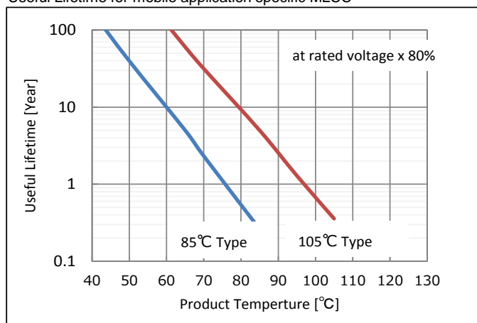
Useful Lifetime for mobile application specific MLCC
