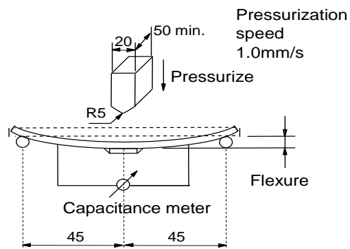
Fig.1 (in mm)
