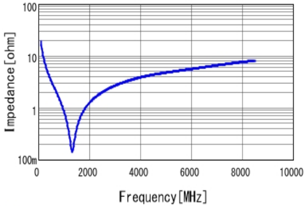
■ GRM0225C1A820JA02 |Z| DCOV, 25degC
