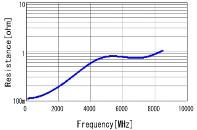
■ GRM0225C1A820JA02 R DCOV, 25degC
