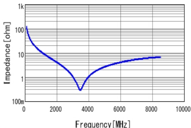
■ GRM0225C1H130GA03 |Z| DC0V, 25degC
