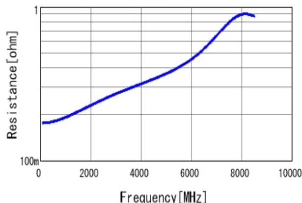
■ GRM0225C1H130GA03 R DC0V, 25degC
