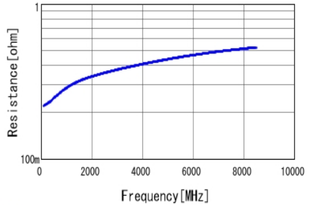
■ GRM0225C1H2R5BA03 R DC0V, 25degC
