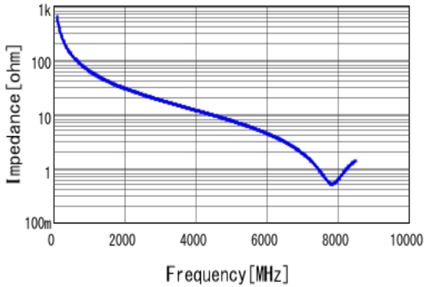
■ GRM0225C1H2R5BA03 |Z| DC0V, 25degC
