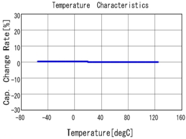
■ GRM2192C1H103JA01 C-Temp. capchange, DCOV, AC1Vrms
