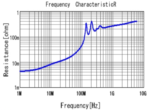
■ GRM2192C1H103JA01 R DCOV, 20degC
