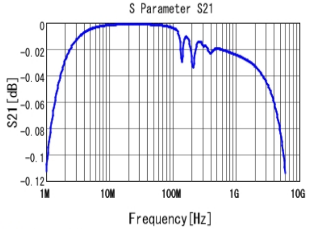
■ GRM2192C1H103JA01 S21 DCOV, 20degC
