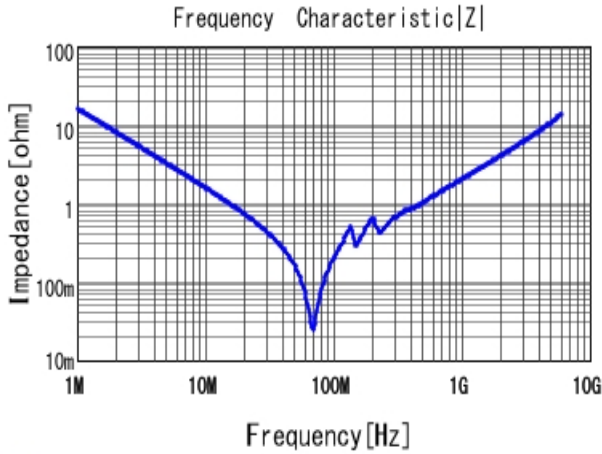
■ GRM2192C1H103JA01 |Z| DCOV, 20degC
