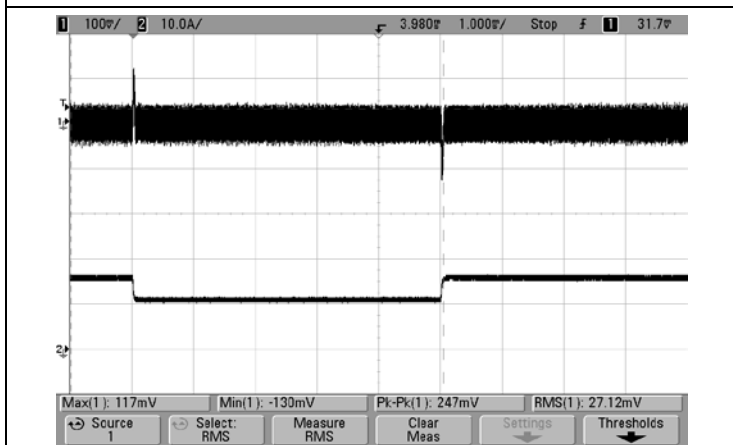
Step Load Transient Response@25°C
