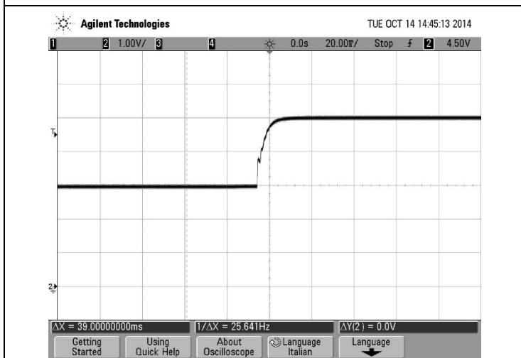
Start-up into a Pre-bias Load@25°C
