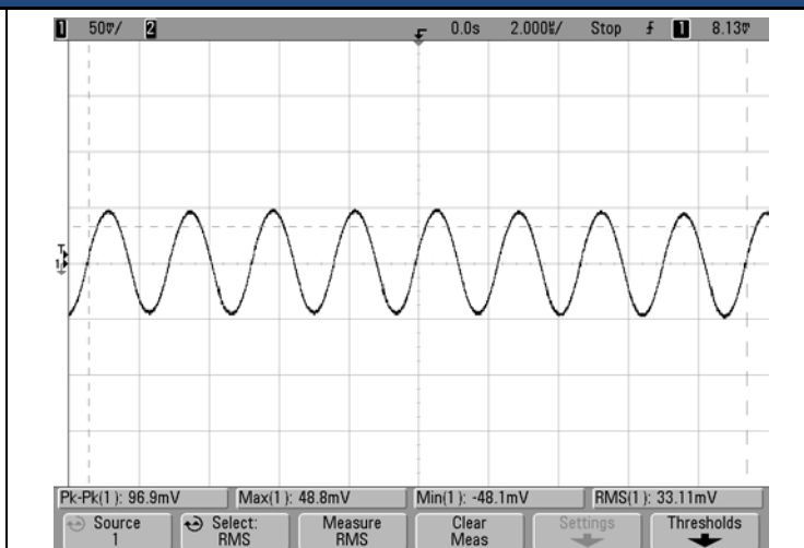
Ripple and Noise @25°C
