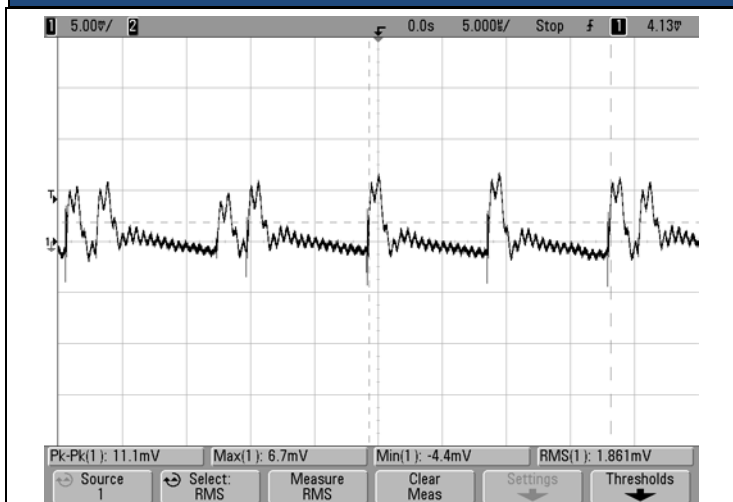
Ripple and Noise @25°C
