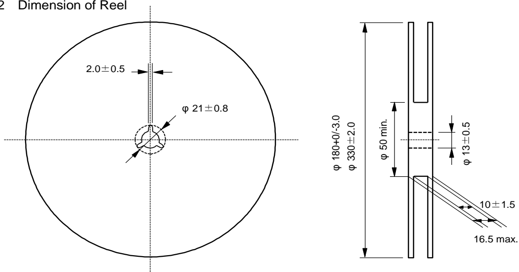
Fig.2 Dimension of Reel
