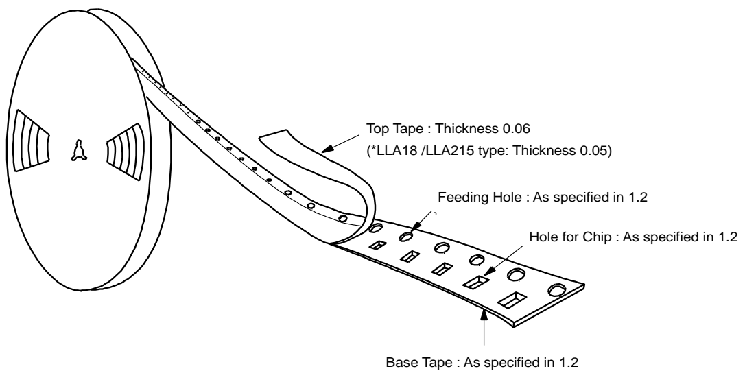
Fig3 Taping Diagram
