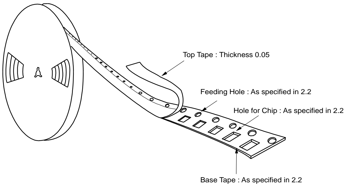
Fig3 Taping Diagram
