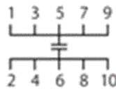
a)Equivalent Circuit
