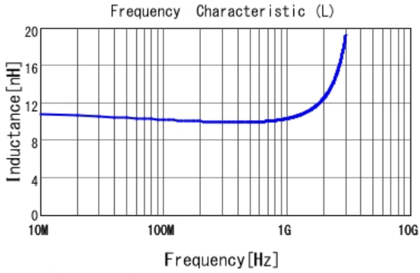
LQG15WH10NG02 L
