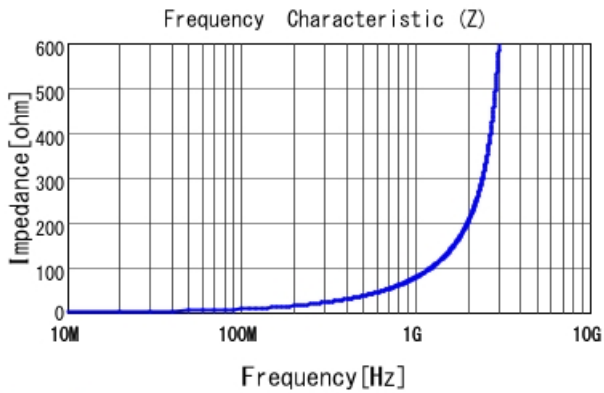
LQG15WH12NG02 |Z|
