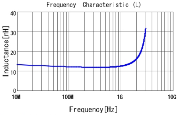
LQG15WH12NG02 L
