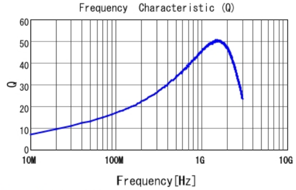
LQG15WH12NG02 Q
