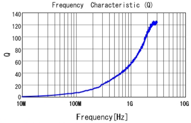
LQG15WH1N0B02 Q
