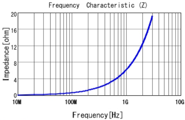
LQG15WH1N0B02 |Z|
