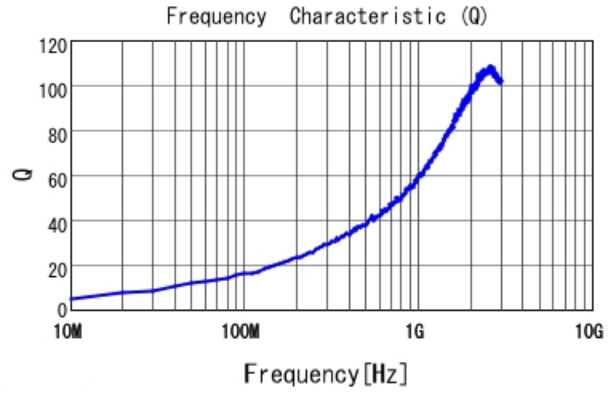
LQG15WH1N6B02 Q
