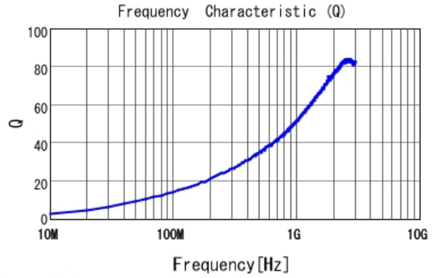
LQG15WH2N4B02 Q
