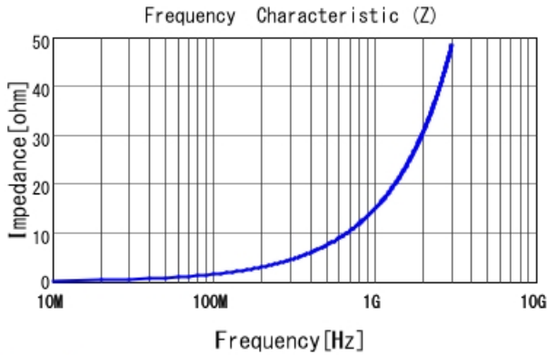
LQG15WH2N4B02 |Z|
