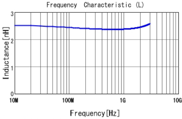
LQG15WH2N4B02 L
