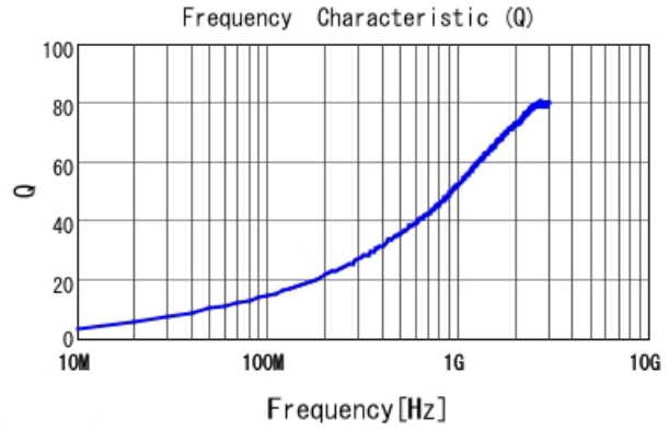
LQG15WH3N0B02 Q
