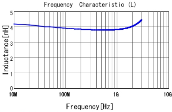
LQG15WH3N9B02 L
