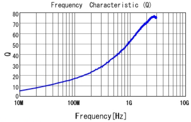
LQG15WH3N9B02 Q
