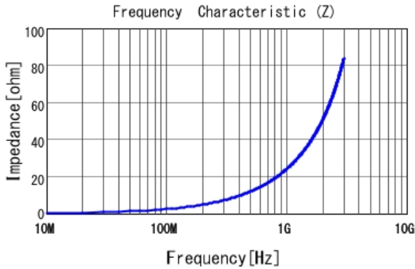
LQG15WH3N9B02 |Z|
