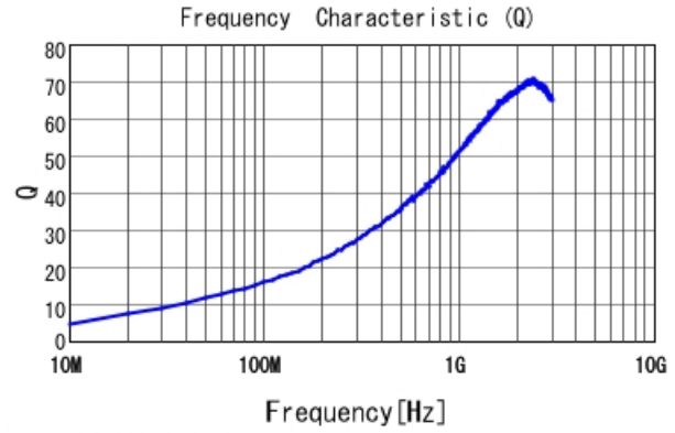
LQG15WH5N1B02 Q
