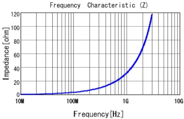
LQG15WH5N1B02 |Z|
