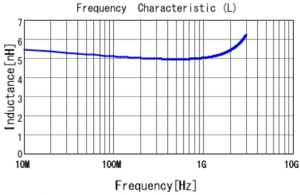
LQG15WH5N1B02 L
