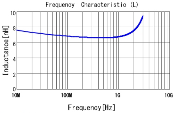
LQG15WH6N8G02 L
