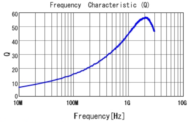
LQG15WH6N8G02 Q
