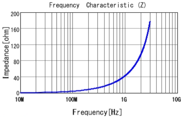
LQG15WH6N8G02 |Z|
