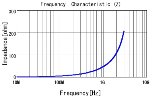
LQG15WH7N5G02 |Z|
