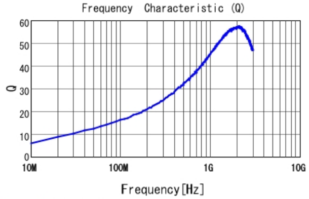
LQG15WH7N5G02 Q
