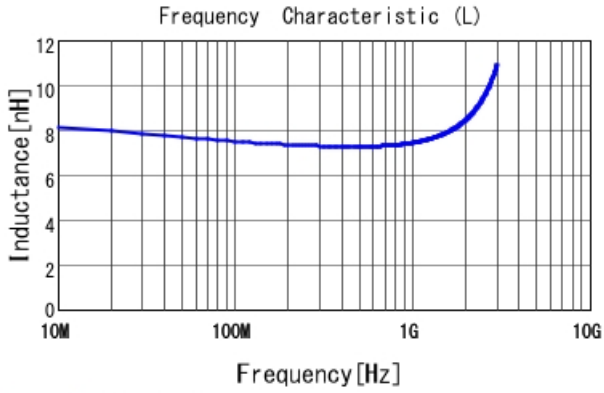
LQG15WH7N5G02 L
