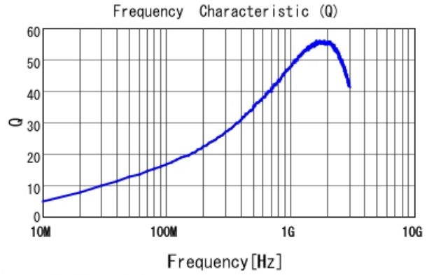
LQG15WH9N1G02 Q
