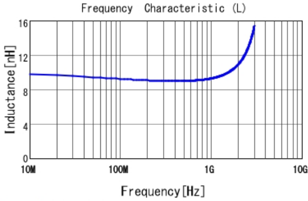
LQG15WH9N1G02 L
