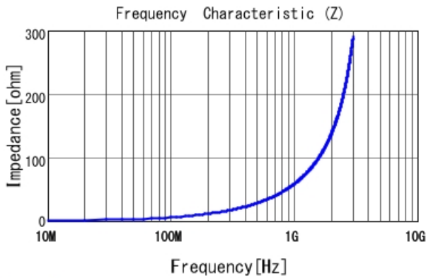
LQG15WH9N1G02 |Z|
