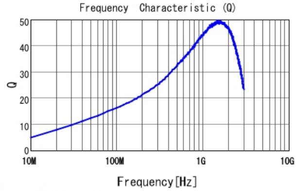
LQG15WZ13NG02 Q
