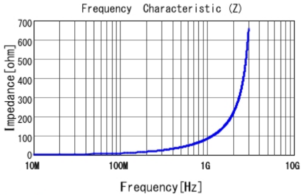
LQG15WZ13NG02 |Z|
