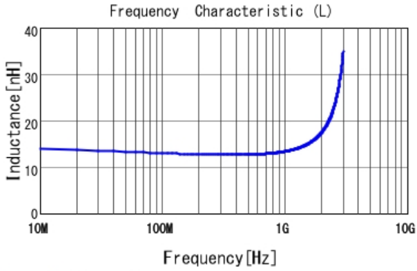
LQG15WZ13NG02 L
