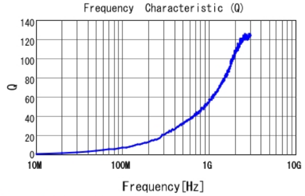
LQG15WZ1N0B02 Q
