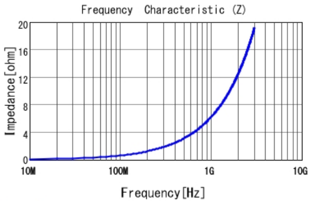
LQG15WZ1N0B02 |Z|
