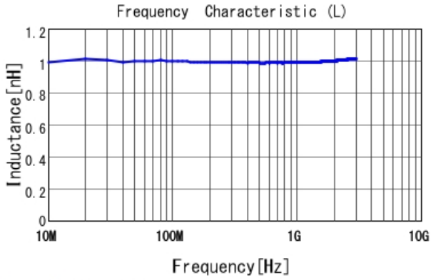
LQG15WZ1N0B02 L
