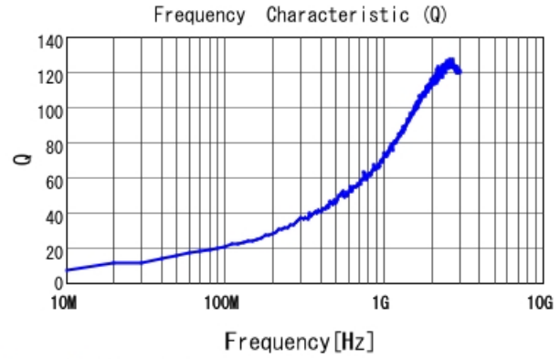
LQG15WZ1N1B02 Q
