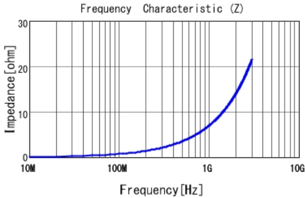
LQG15WZ1N1B02 |Z|
