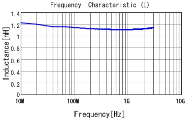
LQG15WZ1N1B02 L
