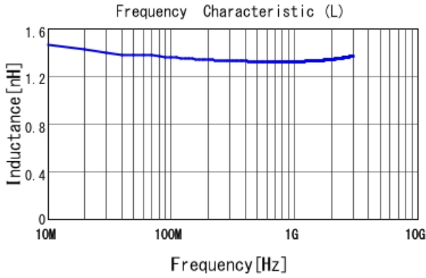
LQG15WZ1N3B02 L
