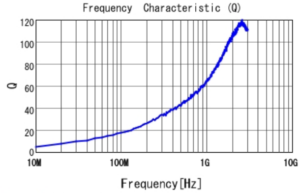
LQG15WZ1N3B02 Q
