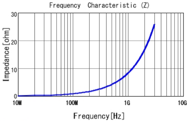
LQG15WZ1N3B02 |Z|
