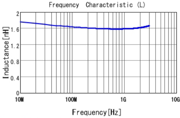
LQG15WZ1N6B02 L
