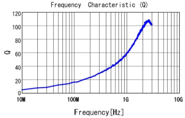
LQG15WZ1N6B02 Q
