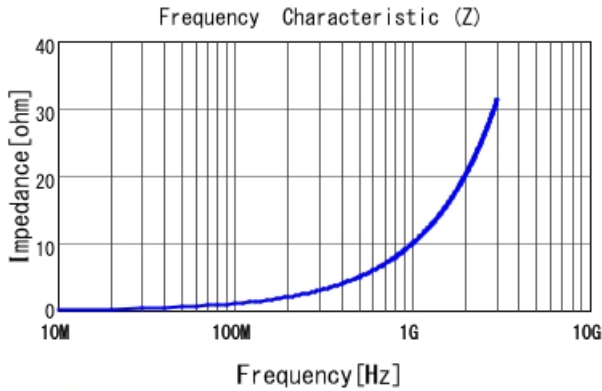
LQG15WZ1N6B02 |Z|
