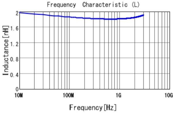
LQG15WZ1N8B02 L
