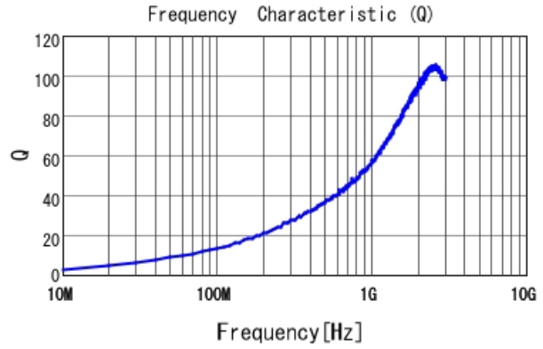
LQG15WZ1N8B02 Q
