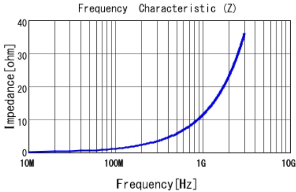
LQG15WZ1N8B02 |Z|
