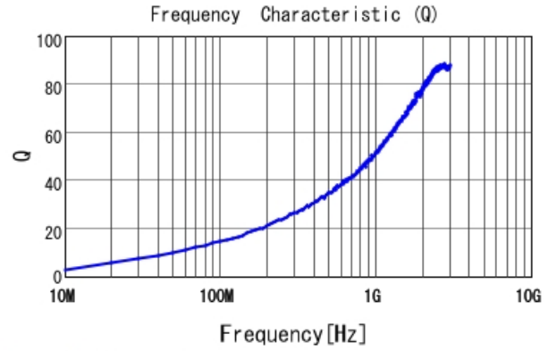
LQG15WZ2N2B02 Q
