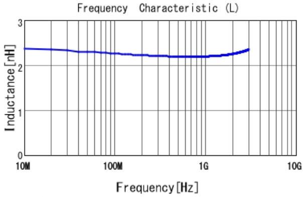
LQG15WZ2N2B02 L
