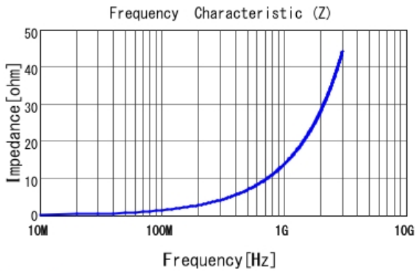
LQG15WZ2N2B02 |Z|
