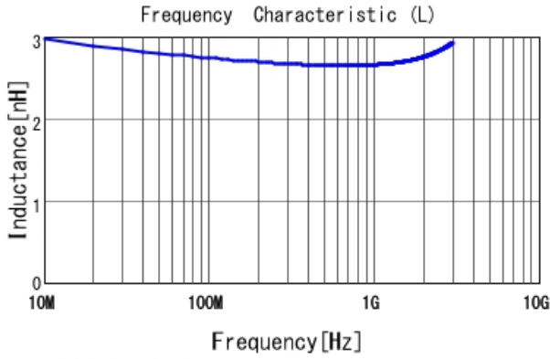
LQG15WZ2N7B02 L
