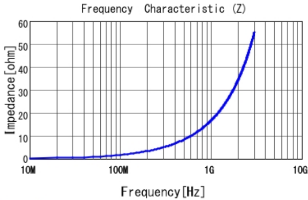
LQG15WZ2N7B02 |Z|
