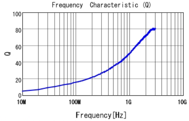
LQG15WZ2N7B02 Q
