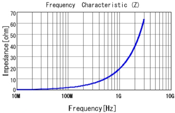
LQG15WZ3N0B02 |Z|
