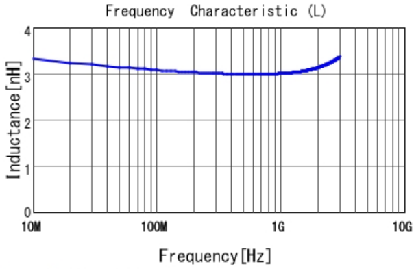
LQG15WZ3N0B02 L
