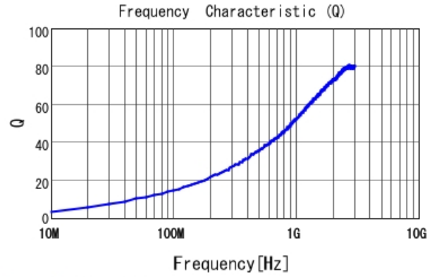
LQG15WZ3N0B02 Q
