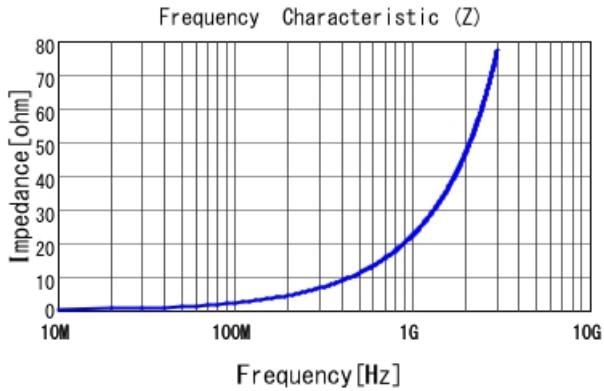
LQG15WZ3N6B02 |Z|
