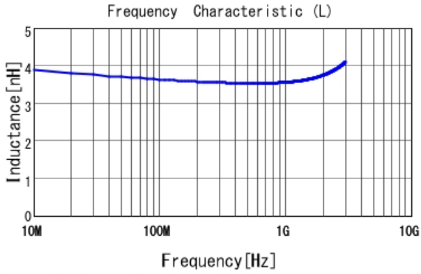
LQG15WZ3N6B02 L
