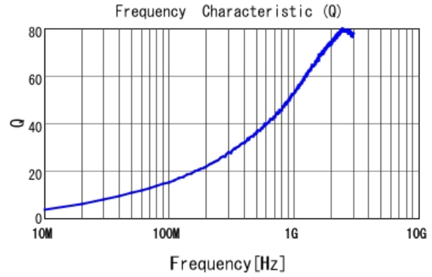
LQG15WZ3N6B02 Q
